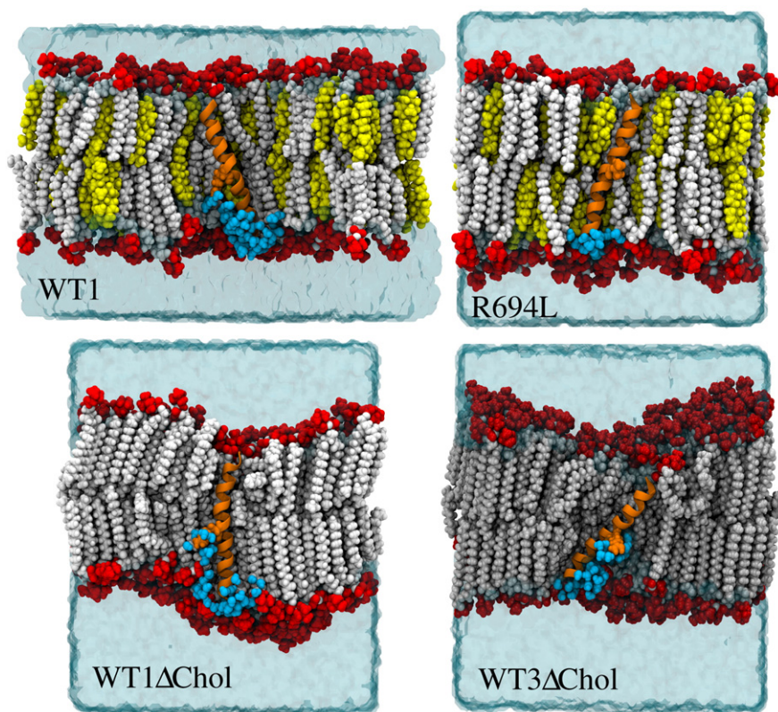
Fig. 4. Representative system configurations from equilibrium MD at 300 ns rendered in VMD [42] for the WT1, R694L, WT1 \Delta Chol, and WT3 \Delta Chol systems. Lipid headgroups are in red vdW, lipid tails in white vdW, cholesterol in yellow vdW, water in cyan isosurface, peptide in orange new cartoon, and R694 or R694L in orange vdW. Water with oxygens within 4 \text{\AA} of the protein and located on the inner leaflet of the membrane are shown in cyan vdW. For clarity, lipids, cholesterol, and water in the foreground of all four configurations are not shown.
