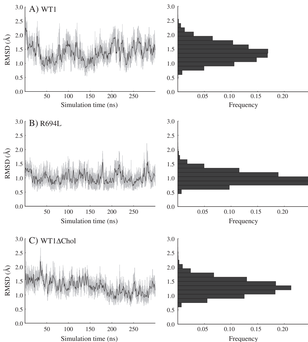
Fig. 2. Collective variable (RMSD of backbone compared to perfect helix) in Å vs. simulation time in ns and histogram of RMSD vs. frequency for equilibrium MD of (A) WT1, (B) R694L, and (C) WT1 \Delta Chol systems.
