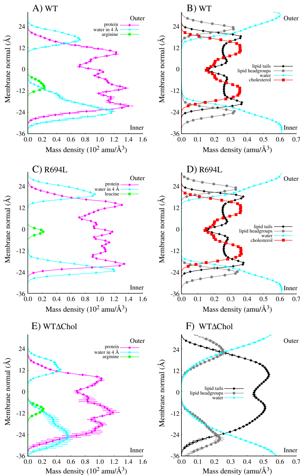
Fig. 3. (A, C, and E) Mass density in 10^2 \text{ amu}/\text{\AA}^3 along membrane normal in Å during equilibrium MD for various components of the system: protein, local water (defined as within 4 Å of protein), and midspan residue (arginine or leucine). (B, D, and F) Mass density in \text{amu}/\text{\AA}^3 along membrane normal in Å during equilibrium MD for various components of the system: lipid tails, lipid headgroups, water, and cholesterol. A and B are averages for WT1, WT2, and WT3 systems. E and F are averages for WT1ΔChol, WT2ΔChol, and WT3ΔChol systems. All statistics are from the last 100 ns of each trajectory and error bars in A, B, E and F represent standard error.
