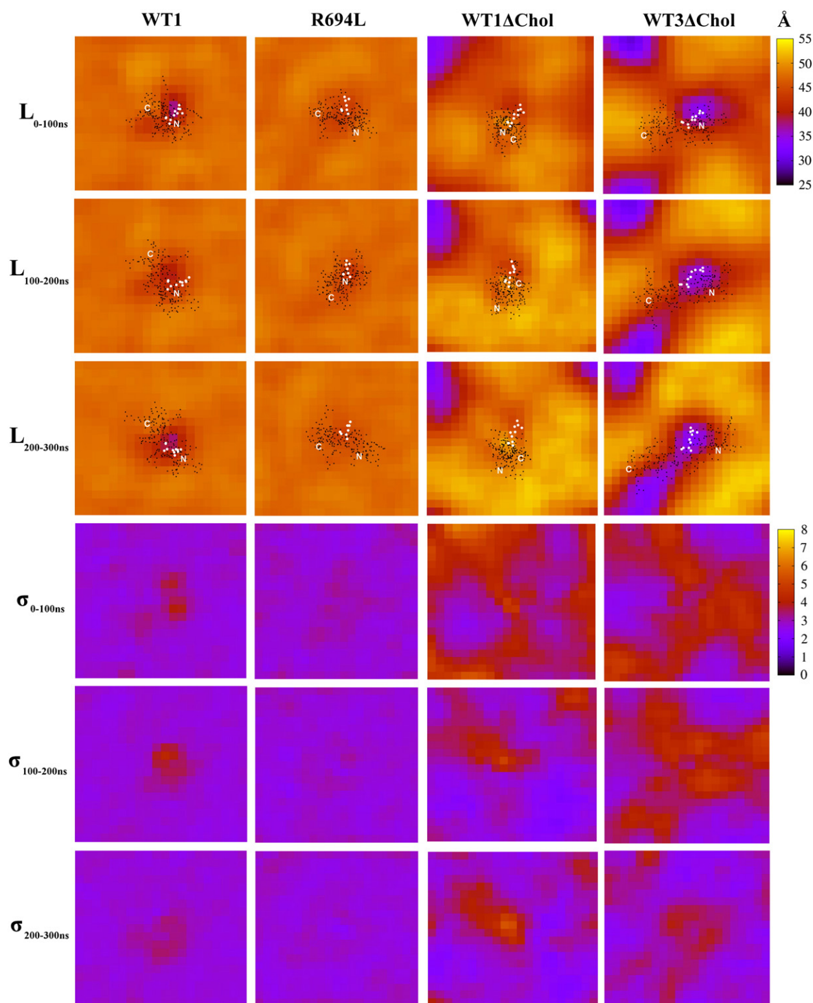
Fig. 7. Maps of membrane thickness, L , (top) in Å and standard deviation, \sigma_L , (bottom) in Å for the WT1, R694L, WT1ΔChol, and WT3ΔChol systems during 100 ns intervals of equilibrium MD. Overlaid on the maps are the x and y positions of the non-hydrogen atoms of the peptide (black circles) and the 694 residue (white circles) from the last frame of the trajectories. The N- and C-termini are labeled.
